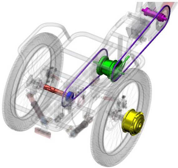
Rear Hub Motor
