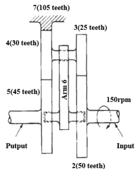
Fig. 4. A planetary gear train
