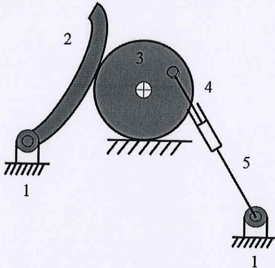
Figure 1(a) Five-bar mechanism
