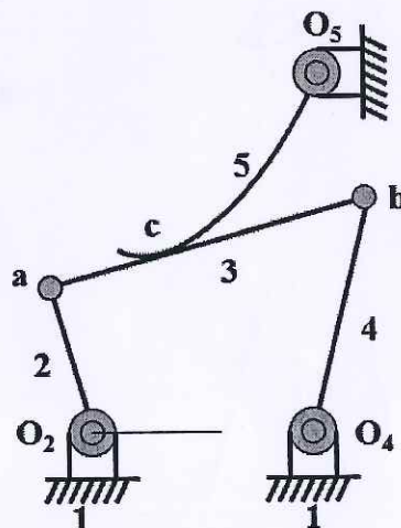
Figure 2(a) Five-bar mechanism
