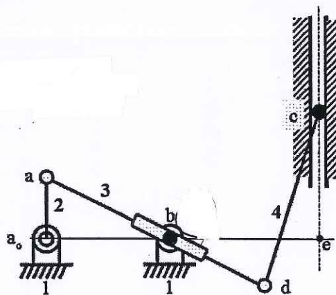
Figure 4 Four-bar mechanism
