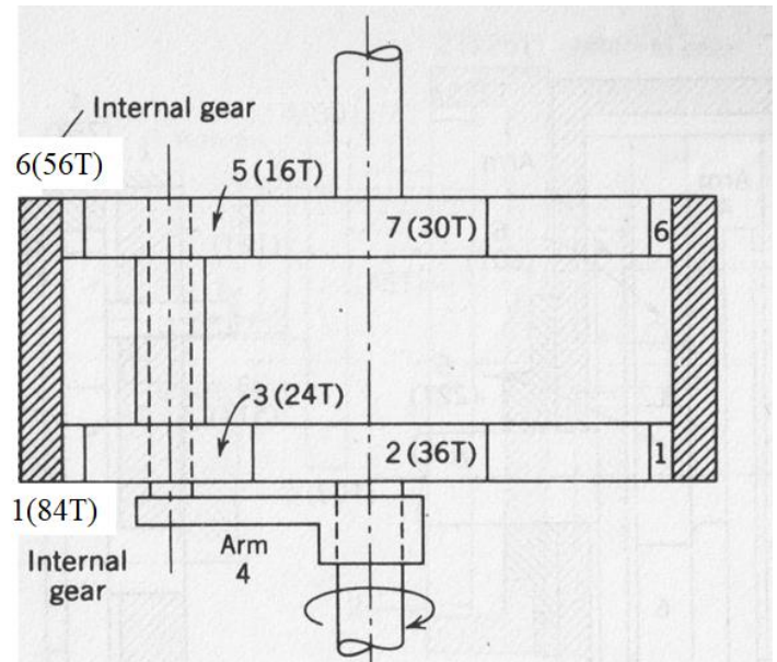
Fig. 4 A planetary gear train
