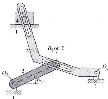
Fig. 2(a) Four-bar mechanism
