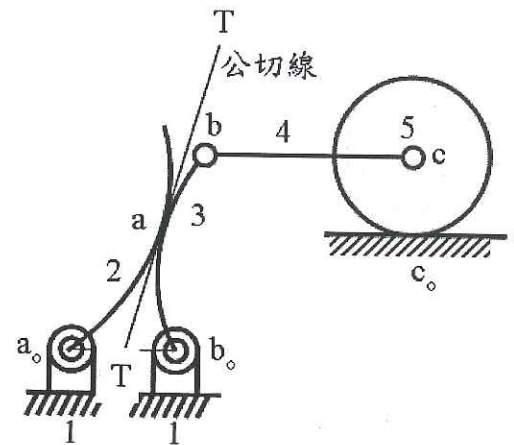
Fig. 2(b) Five-bar mechanism
