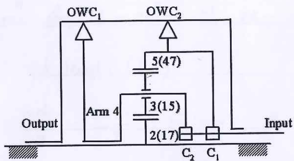
Figure 3 3-speed internal gear hub
