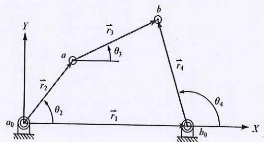
Fig. 1 Four-bar linkage
